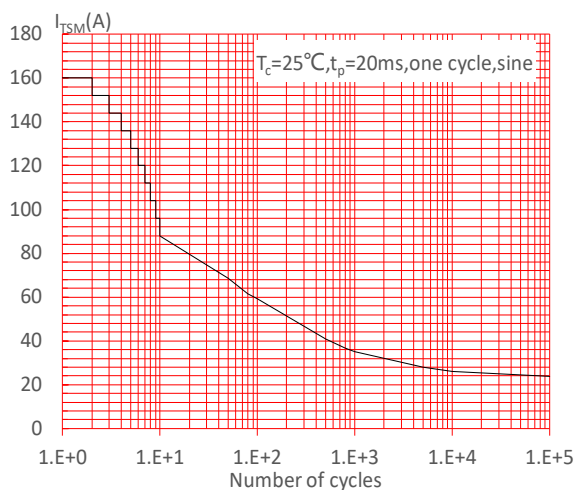
FIG.5: Non-repetitive surge peak on-state current for a sinusoidal pulse with width t_p < 20ms , and corresponding value of I^2t ( di/dt < 80A/\mu s )
