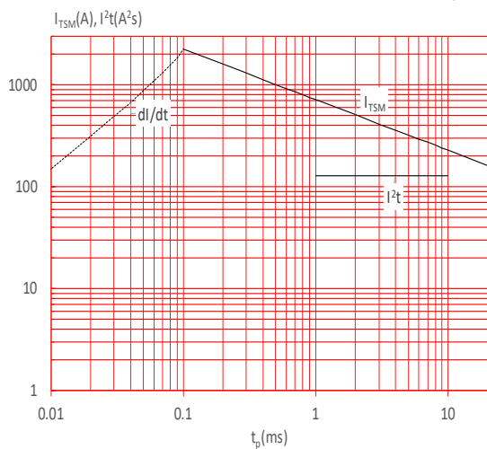
FIG.5: Non-repetitive surge peak on-state current for a sinusoidal pulse with width t_p < 20ms , and corresponding value of I^2t ( di/dt < 80A/\mu s )
