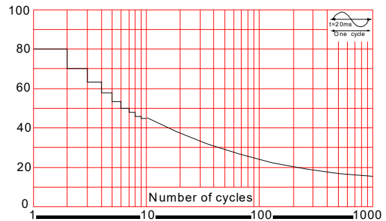
FIG.6: Non-repetitive surge peak on-state current for a sinusoidal pulse with width tp<20ms, and corresponding value of I't (di/dt <50A/μs)
