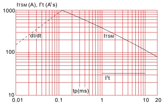
FIG.6: Non-repetitive surge peak on-state current for a sinusoidal pulse with width tp<20ms, and corresponding value of I't (di/dt <50A/μs)
