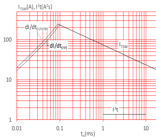
FIG.6: Non-repetitive surge peak on-state current for a sinusoidal pulse with width t_p < 20ms , and corresponding value of I^2t ( I - II - III: di/dt < 50A/\mu s ; IV: di/dt < 30A/\mu s )
