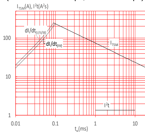
FIG.6: Non-repetitive surge peak on-state current for a sinusoidal pulse with width t_p < 20\text{ms} , and corresponding value of I^2t ( I - II - III: di/dt < 50\text{A}/\mu\text{s} ; IV: di/dt < 30\text{A}/\mu\text{s} )
