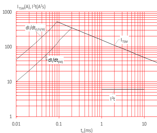
FIG.5: Non-repetitive surge peak on-state current for a sinusoidal pulse with width t_p < 20ms , and corresponding value of I^2t (I - II - III: dl/dt < 50A/\mu s ; IV: dl/dt < 40A/\mu s )
