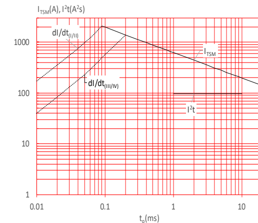
FIG.6: Non-repetitive surge peak on-state current for a sinusoidal pulse with width t_p < 20ms , and corresponding value of I^2t (I - II: di/dt < 100A/\mu s ; III-IV: di/dt < 70A/\mu s )
