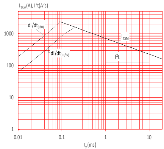
FIG.6: Non-repetitive surge peak on-state current for a sinusoidal pulse with width t_p < 20\text{ms} , and corresponding value of I^2t ( I - II: dl/dt < 80\text{A}/\mu\text{s} ; III-IV: dl/dt < 40\text{A}/\mu\text{s} )
