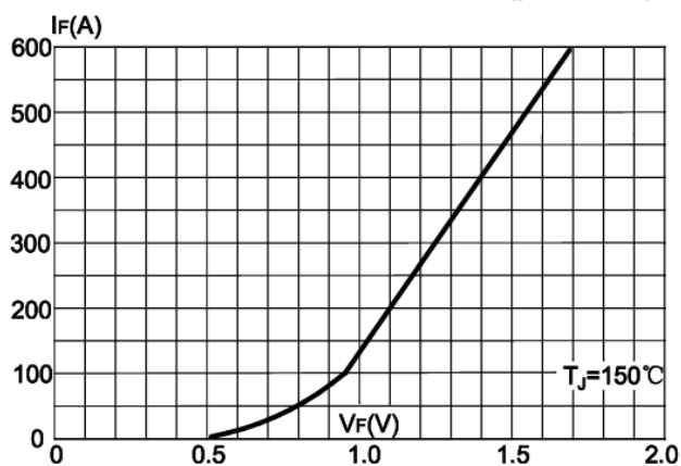
FIG.1: Forward characteristics(per diode)
