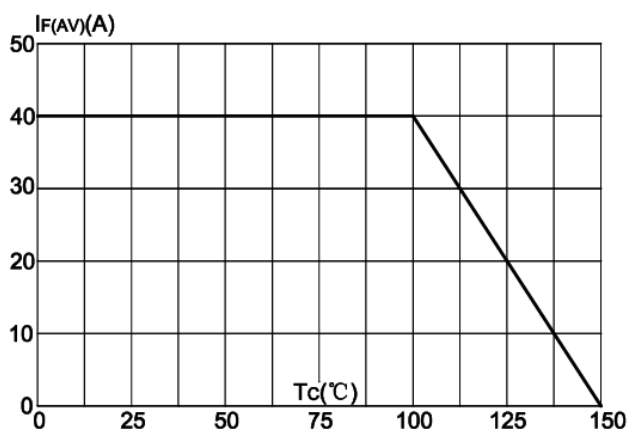
FIG.3: Forward current vs. case temperature
