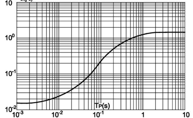
FIG.4: Maximum transient thermal impedance R_{th(j-c)} ( ^\circ\text{C/W} ) Junction-to-case(per diode)
