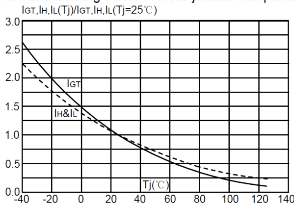
FIG.4: Relative variations of gate trigger current, holding current and latching current versus junction temperature I_{GT}, I_H, I_L(T_j)/I_{GT}, I_H, I_L(T_j=25^\circ\text{C})
