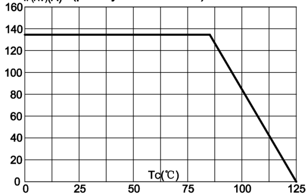
FIG.6: Forward current vs. case temperature I_{F(AV)} (per thyristor or diode)
