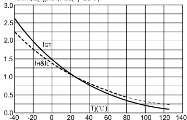
FIG.4: Relative variations of gate trigger current, holding current and latching current versus junction temperature IGT,IH,IL(TJ)/IGT,IH,IL(TJ=25°C)
