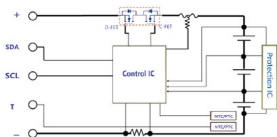
High-side Configuration
